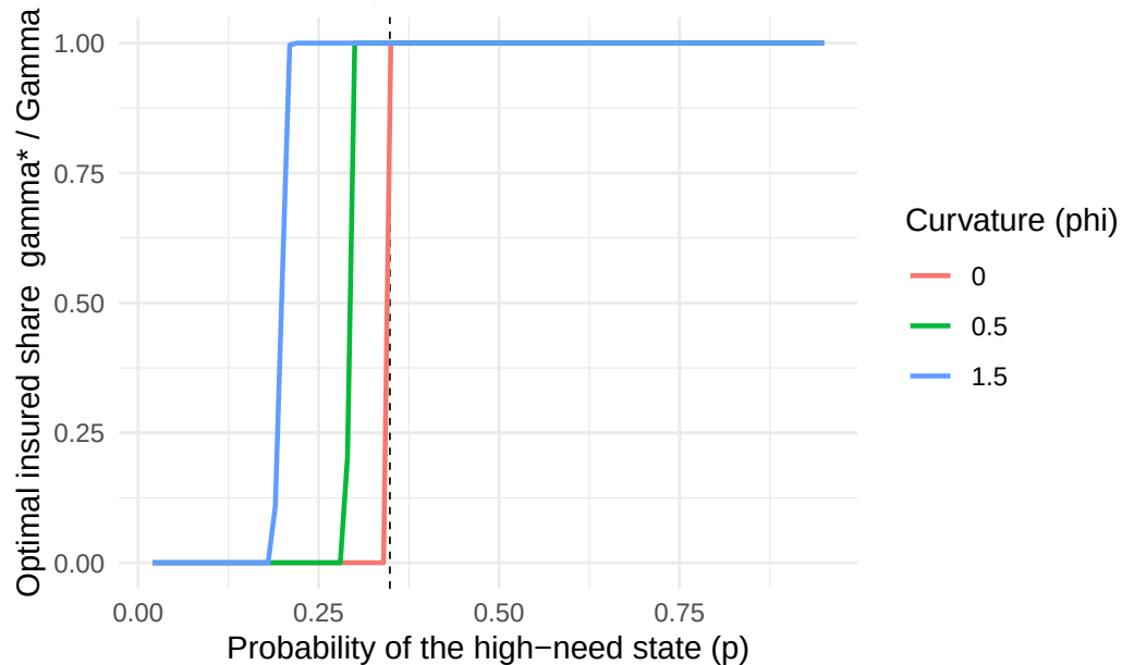
The normative policy function
