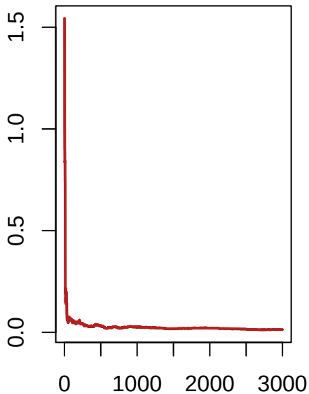
Estimation error \|\theta_{\text{hat}} - \theta^*\|
