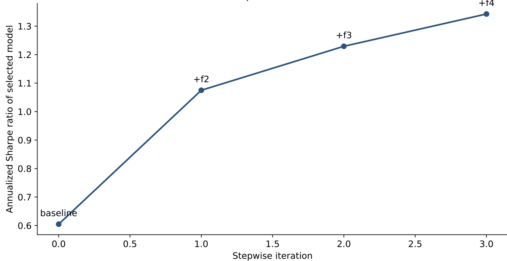
Efficient-frontier expansion as factors are added
