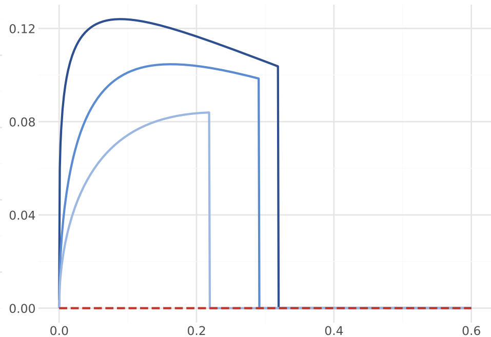
Experts' wealth share \eta
