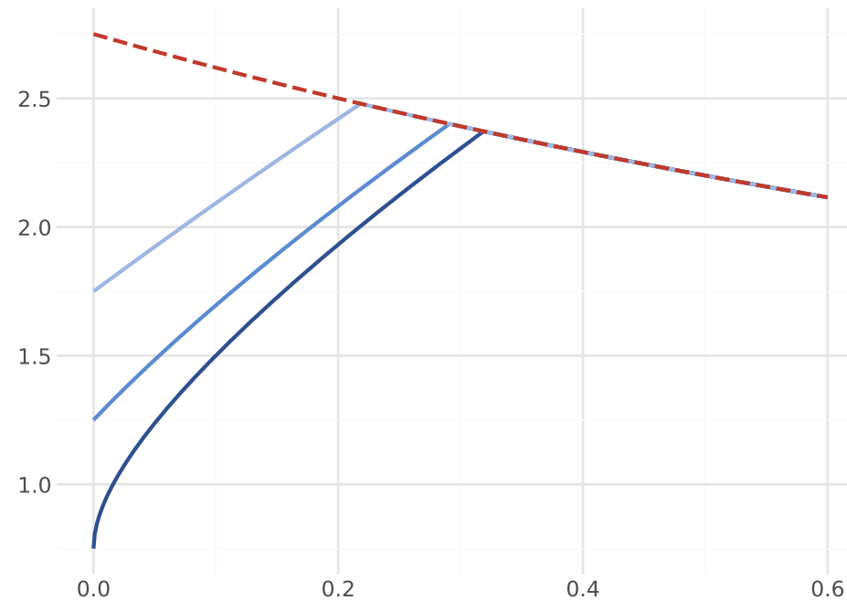
Experts' wealth share \eta
