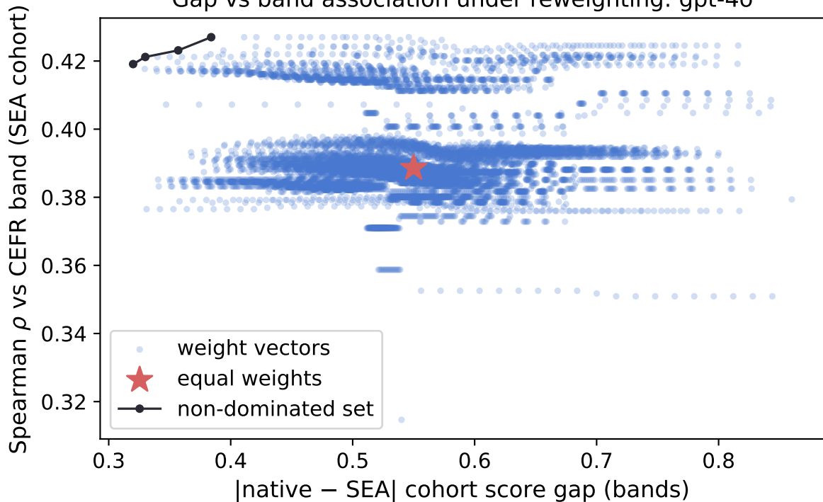
Gap vs band association under reweighting: gpt-4o
