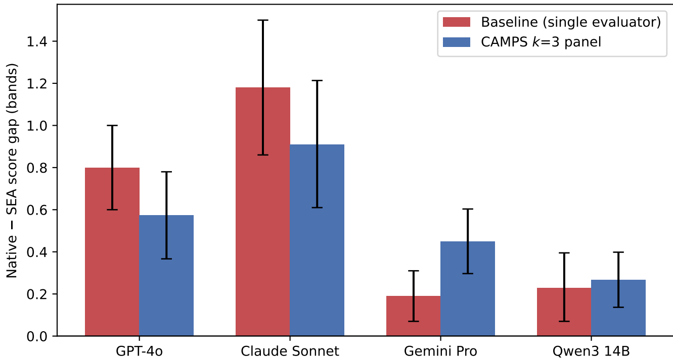
Cohort score gap by model and condition (95% bootstrap CIs, n=100 /cohort)
