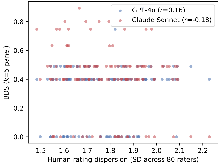
BDS vs human dispersion (all 136 matched essays)
