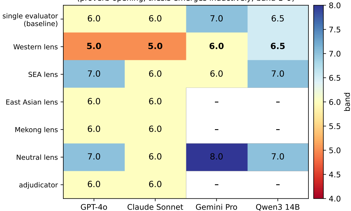
One essay, every lens: WE_PHL_PTJ0_087_B1_2 (proverb opening, thesis emerges inductively; band 1-9)
