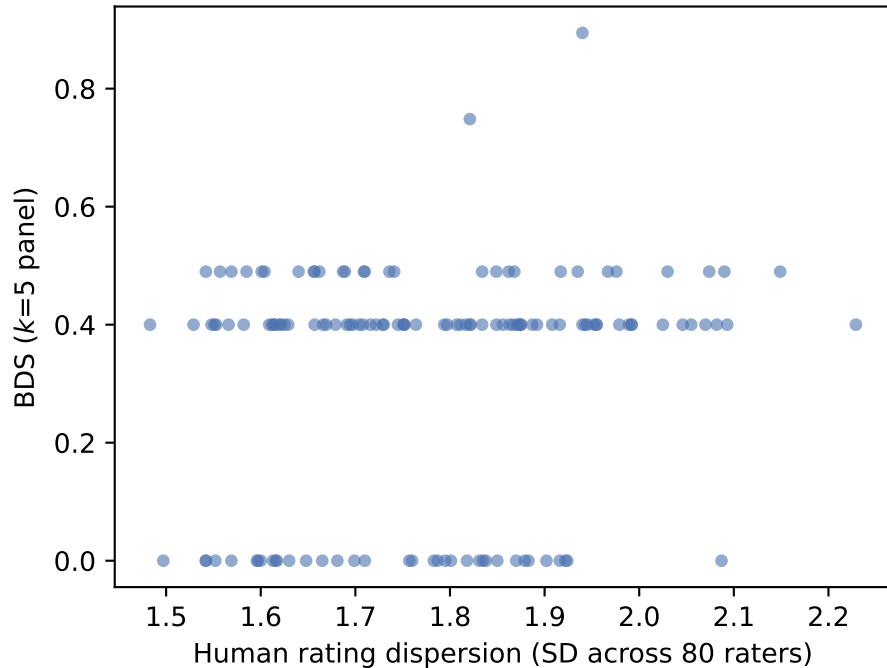
BDS vs human dispersion ( n=136 , r=0.16 )
