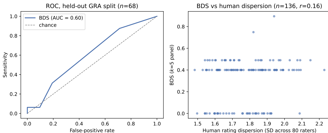
Figure 4-4: Left: ROC of BDS against top-quartile human dispersion on the held-out GRA split (GPT-4o panel). Right: BDS against the dispersion of 80 human raters; the discreteness of BDS under integer lens scores is visible as horizontal bands.
