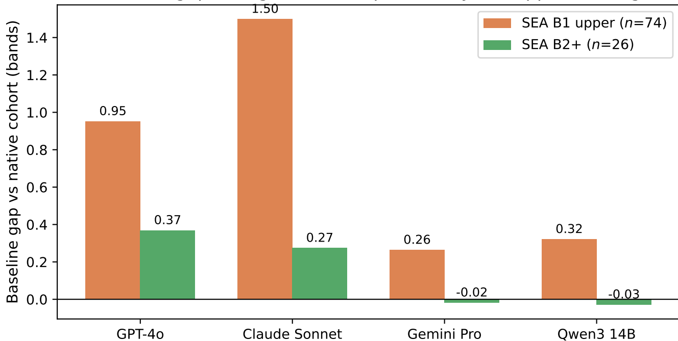
Baseline gap is largest for mid-proficiency (B1 upper) writing
