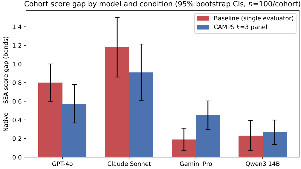
Figure 4-1: Native-SEA score gap by model and condition, with 95% bootstrap confidence intervals ( n=100 per cohort). Every baseline gap excludes zero; the panel narrows the gap on the two models where it is largest, leaves it unchanged on Qwen3, and widens it on Gemini Pro.
