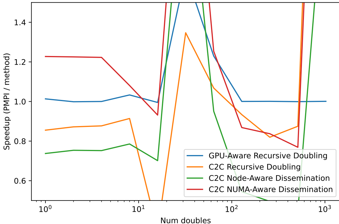
Allreduce Speedup vs PMPI 64 nodes, PPG=1
