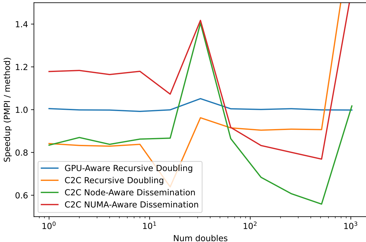
Allreduce Speedup vs PMPI 8 nodes, PPG=1
