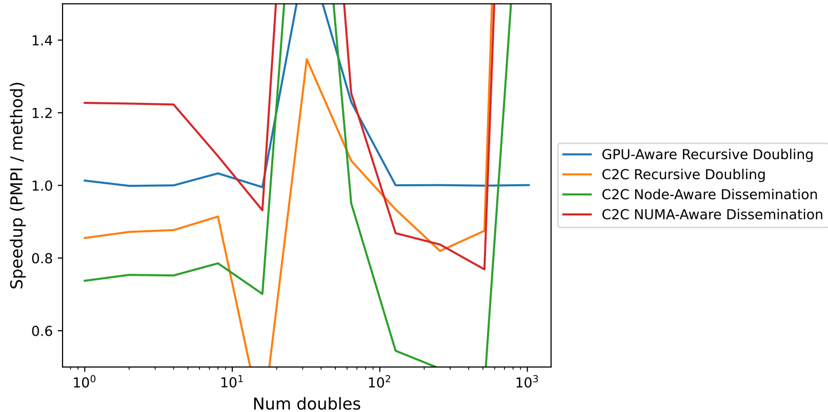
Allreduce Speedup vs PMPI 64 nodes, PPG=1
