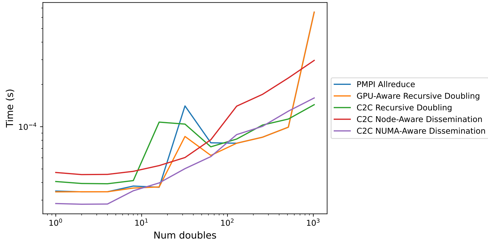
Allreduce Timings 64 nodes, PPG=1
