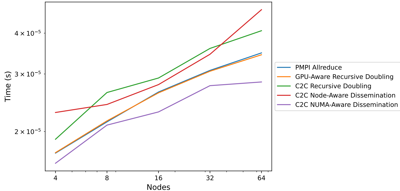
Allreduce Timings vs Nodes Smallest Size (1 doubles), PPG=1
