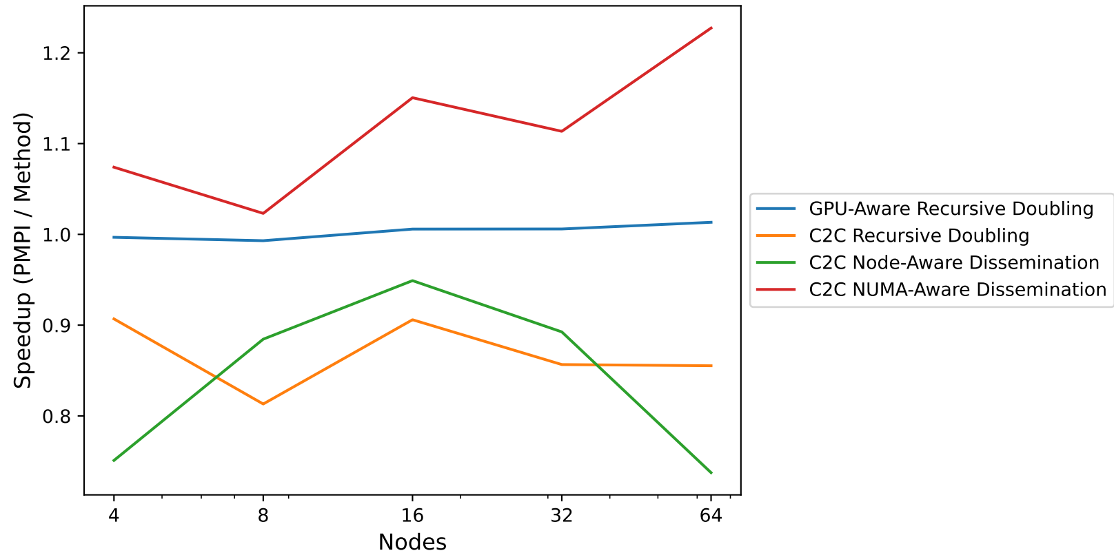
Allreduce Speedup vs PMPI Smallest Size (1 doubles), PPG=1
