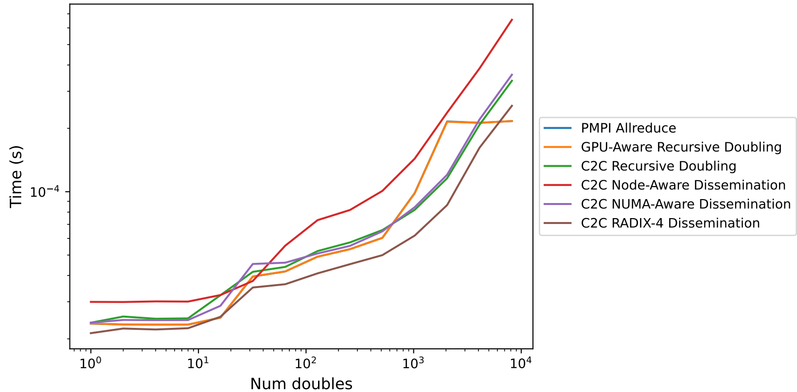
Allreduce Timings 32 nodes, PPG=1
