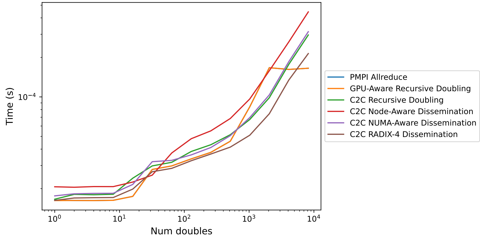
Allreduce Timings 8 nodes, PPG=1
