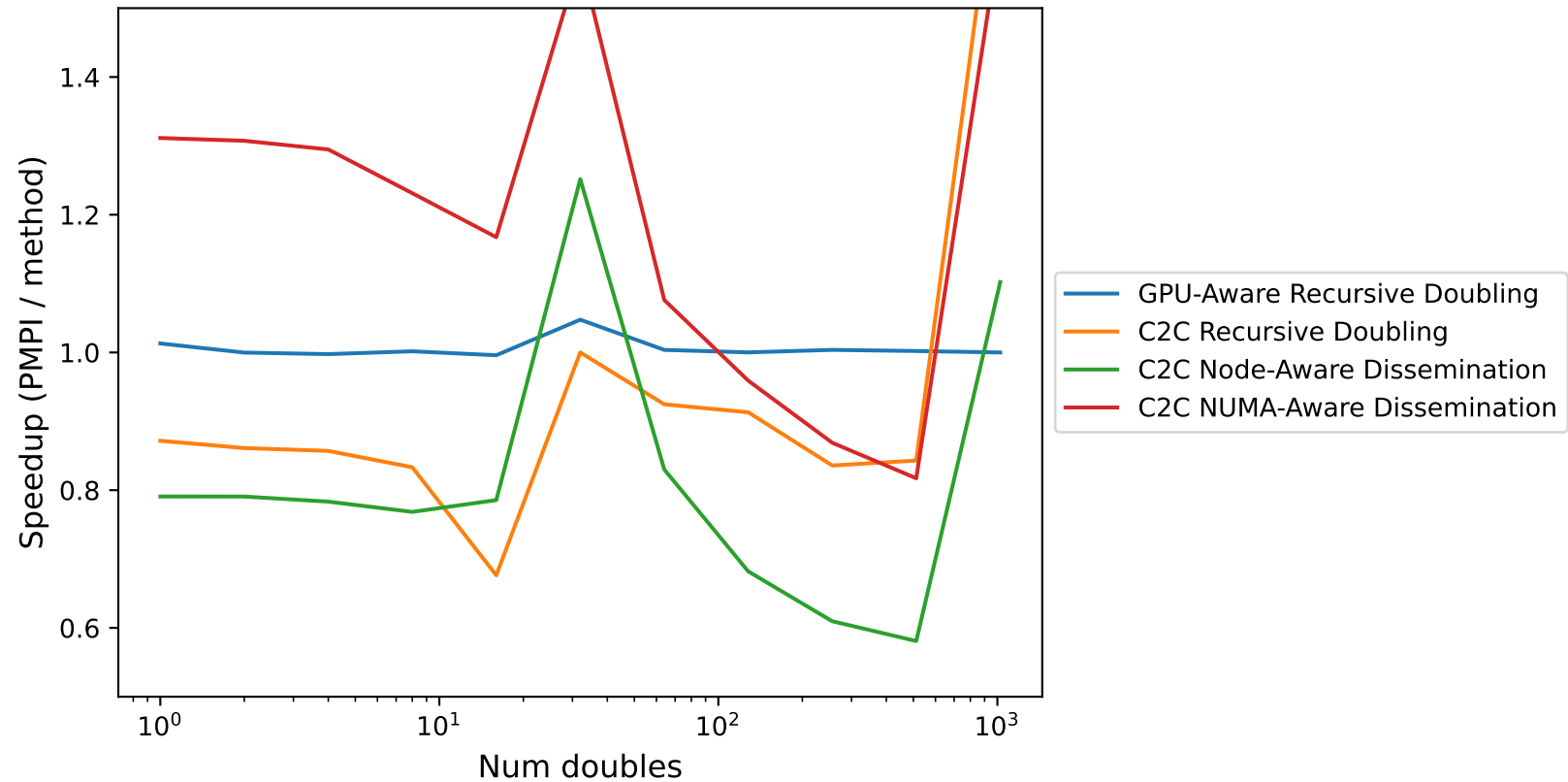
Allreduce Speedup vs PMPI 16 nodes, PPG=1
