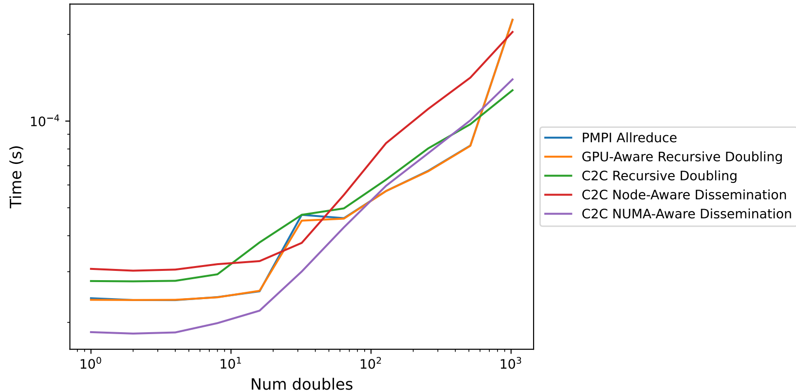
Allreduce Timings 16 nodes, PPG=1
