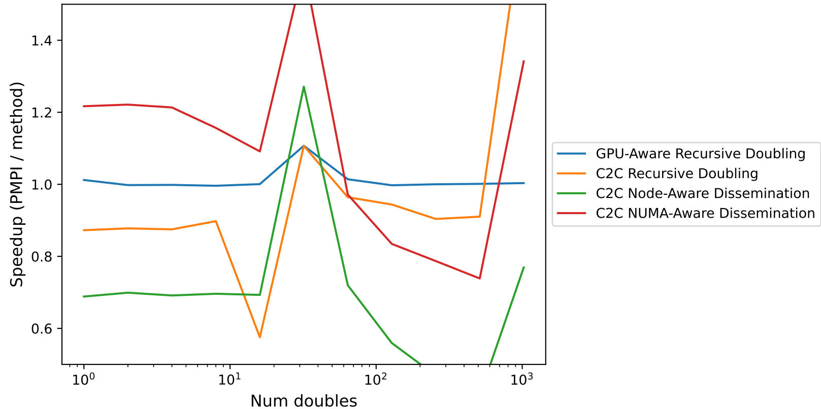
Allreduce Speedup vs PMPI 32 nodes, PPG=1
