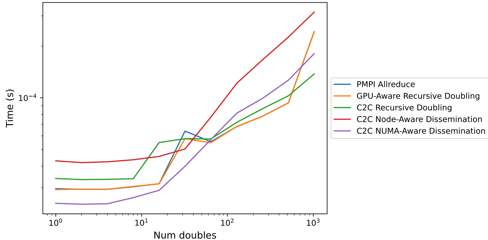
Allreduce Timings 32 nodes, PPG=1
