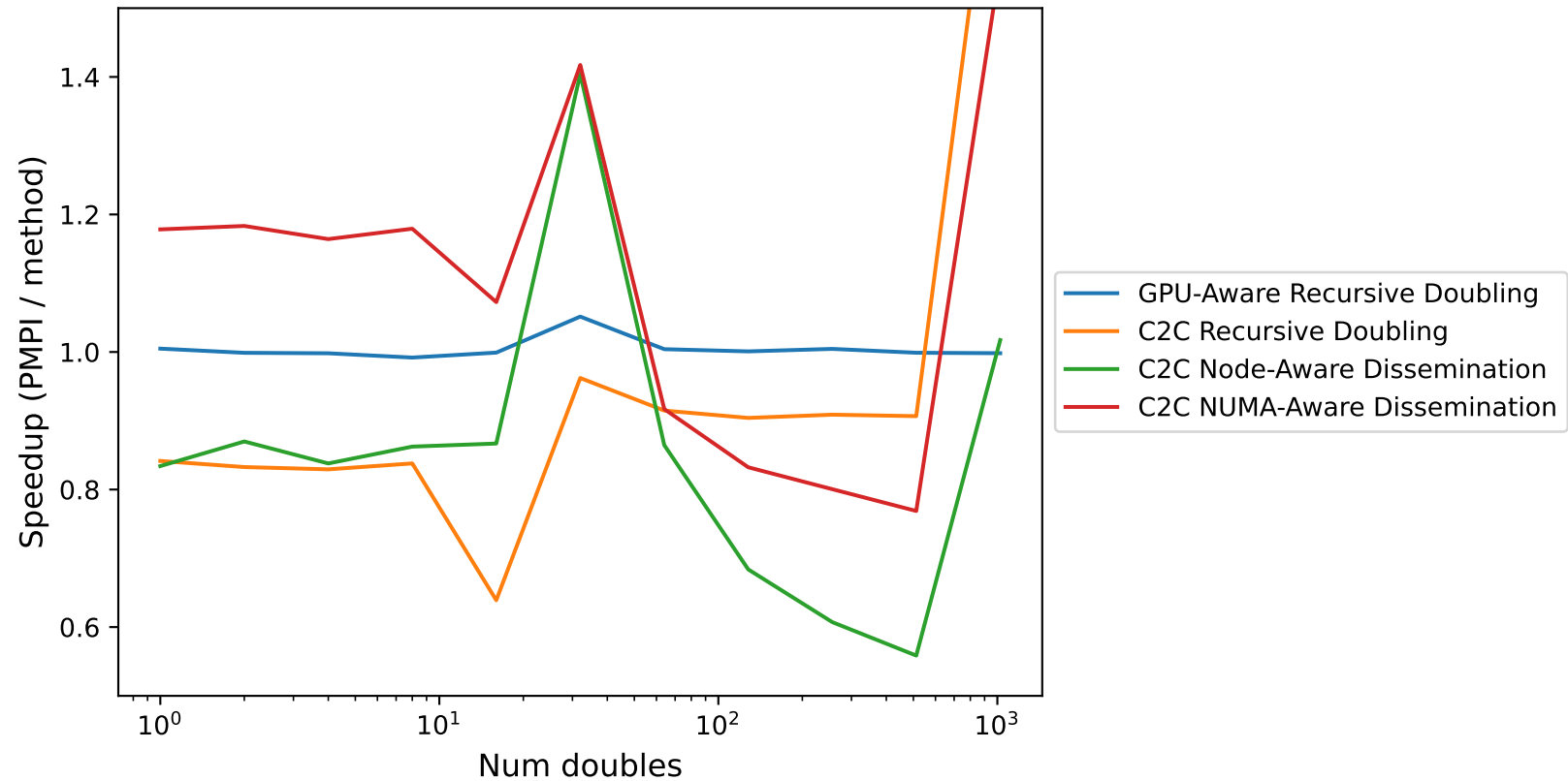
Allreduce Speedup vs PMPI 8 nodes, PPG=1
