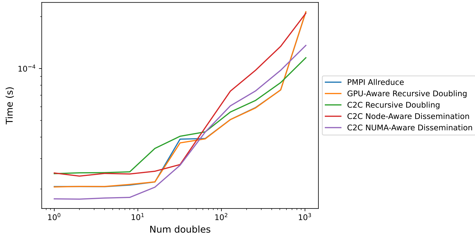
Allreduce Timings 8 nodes, PPG=1
