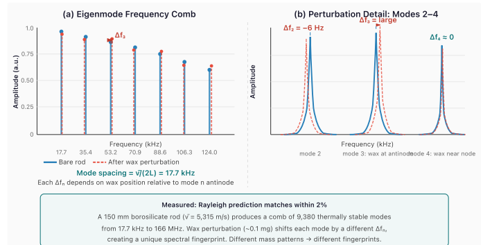
Figure 11. (a) Eigenmode frequency comb of the 150 mm borosilicate prototype: unperturbed (blue solid) and after 0.1 mg wax perturbation (red dashed). Each mode shifts by a different \Delta f_n , depending on the wax position relative to that mode’s antinode. (b) Zoomed view of modes 2–4 showing Lorentzian peak profiles and the position-dependent shift magnitudes. Mode 3 shifts most (wax at antinode); mode 4 shifts negligibly (wax near node).
