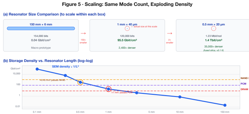
Figure 5. (a) Size comparison at three scales: the 150 mm macro prototype (0.04 Gbit/cm 3 ), the 1 mm borosilicate MEMS rod (95.5 Gbit/cm 3 , 2,400× denser), and a 0.5 mm fused silica array (1.4 Tbit/cm 3 , 35,000× denser). All designs share the same thermally stable mode physics. (b) Log-log density vs. rod length showing SEM crossing DRAM at 2.1 mm, PCM at 1.0 mm, and NAND Flash at 0.45 mm—all within standard MEMS fabrication range.
