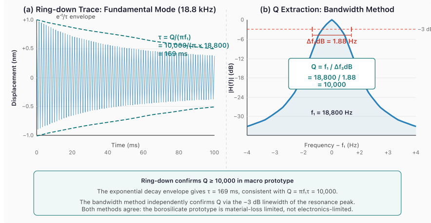
Figure 12. (a) Ring-down waveform of the fundamental mode (18.8 kHz) after impulse excitation. The exponential envelope decays with \tau = 169 \text{ ms} , corresponding to Q = 10,000 . (b) Frequency-domain measurement: the -3 \text{ dB} bandwidth of the Lorentzian resonance peak is 1.88 \text{ Hz} , independently confirming Q = f_r / \Delta f_{\text{dB}} = 10,000 . Both methods agree that the prototype is material-loss-limited.
