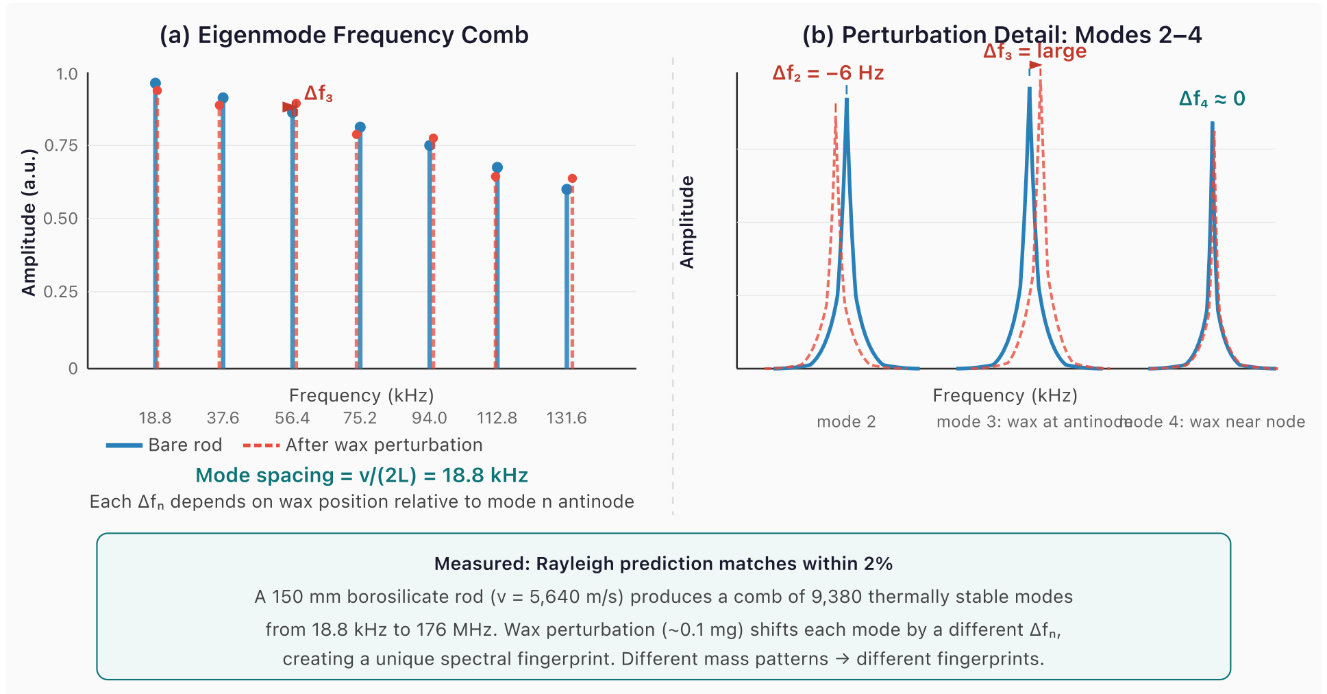
Figure 11. Eigenmode frequency comb of the 150 mm borosilicate prototype. (a) Unperturbed spectrum (blue solid) shows a clean comb at 18.8 kHz spacing. After 0.1 mg wax perturbation (red dashed), each mode shifts by a different \Delta f_n depending on the wax position relative to that mode's antinode — the spectral fingerprint of the perturbation. (b) Zoomed view of modes 2–4 showing Lorentzian peak profiles and position-dependent shift magnitudes. Mode 3 shifts most (wax at antinode); mode 4 barely shifts (wax near node). Measured shifts match Rayleigh predictions to within 2%.
