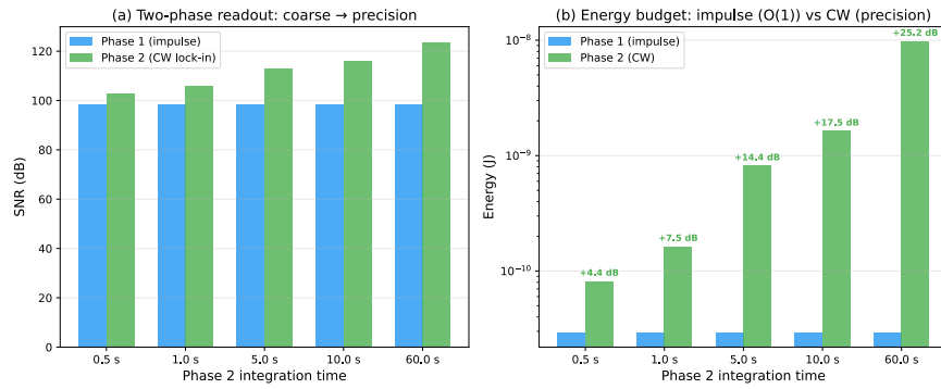
Figure 16. Two-phase readout architecture: Phase 1 (broadband impulse) performs parallel search across all rods in one ring-down time \tau ; Phase 2 (CW lock-in) provides precision measurement on the winning rod at +17.5 dB SNR gain.
