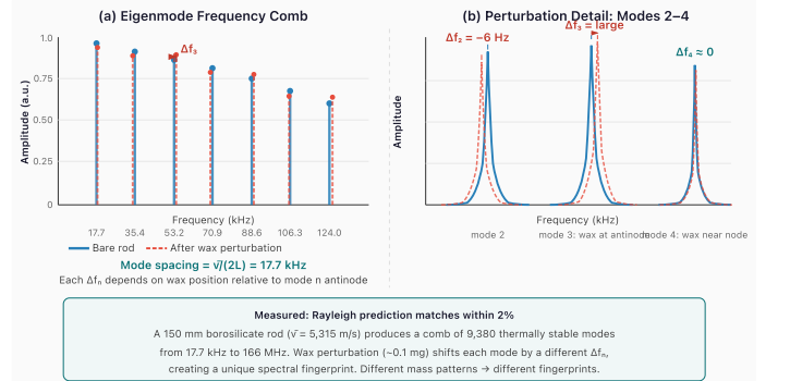
Figure 11. (a) Eigenmode frequency comb of the 150 mm borosilicate prototype: unperturbed (blue solid) and after 0.1 mg wax perturbation (red dashed). Each mode shifts by a different \Delta f_n depending on the wax position relative to that mode’s antinode. (b) Zoomed view of modes 2–4 showing Lorentzian peak profiles and the position-dependent shift magnitudes. Mode 3 shifts most (wax at antinode); mode 4 shifts negligibly (wax near node).
