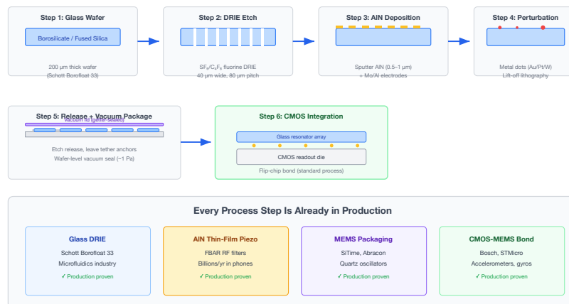
Figure 6. Six-step fabrication process using established MEMS production techniques. The innovation is the architectural combination, not the fabrication.
