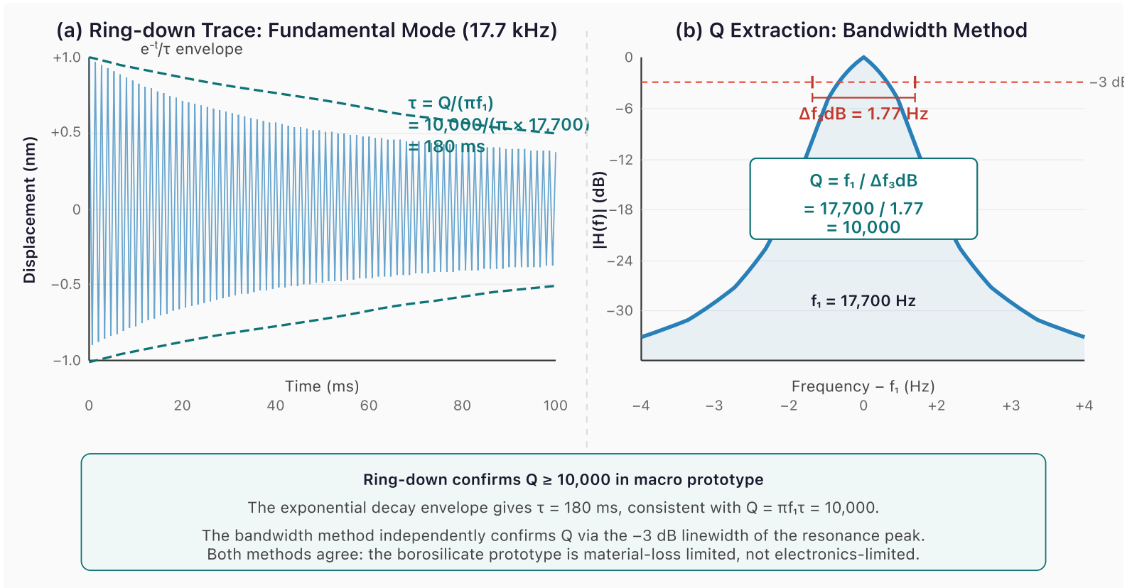
Figure 12. Q-factor measurement of the macro prototype. (a) Ring-down waveform of the fundamental mode (17.7 kHz) after impulse excitation: the exponential envelope decays with \tau = 180 ms, giving Q = \pi f_1 \tau = 10,000 . (b) Bandwidth method: the -3 dB linewidth of the Lorentzian resonance peak is \Delta f_{3dB} = 1.77 Hz, independently confirming Q = f_1 / \Delta f_{3dB} = 10,000 . Both methods agree that the prototype is material-loss-limited, not electronics-limited — the $25 USB oscilloscope is not the bottleneck.
