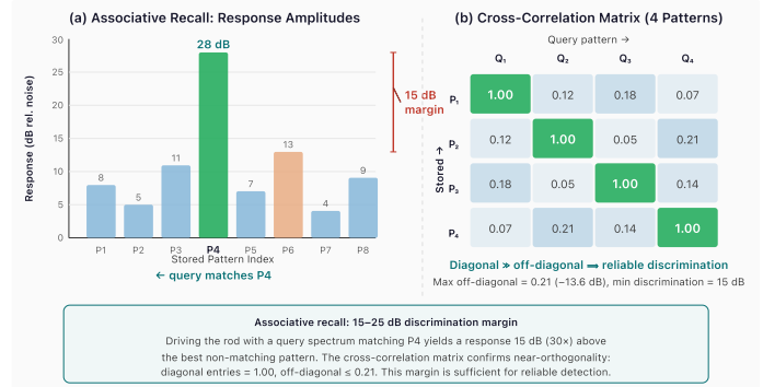
Figure 13. (a) Response amplitudes when querying for pattern P4 across an 8-pattern array. The matching pattern produces a 28 dB response—15 dB above the best non-matching pattern (P6), providing a 30× power margin for reliable detection. (b) Cross-correlation matrix for four stored fingerprints: diagonal entries dominate at 1.00, off-diagonal entries \leq 0.21 , confirming spectral orthogonality.
