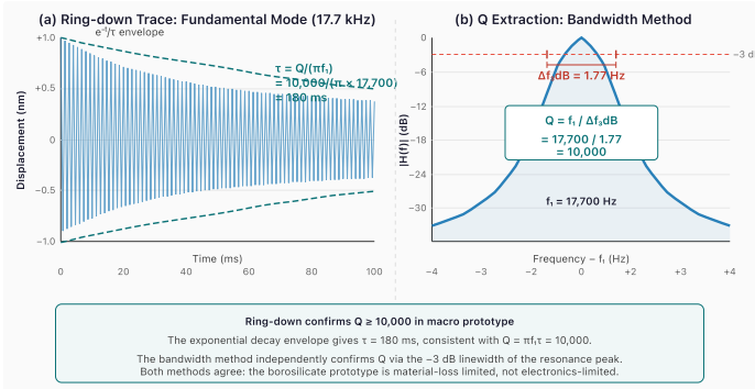
Figure 12. (a) Ring-down waveform of the fundamental mode (17.7 kHz) after impulse excitation. The exponential envelope decays with \tau \approx 180 \text{ ms} , corresponding to Q \approx 10,000 . (b) Frequency-domain measurement: the -3 \text{ dB} linewidth of the Lorentzian resonance peak is 1.77 Hz, independently confirming Q = f_r/\Delta f_{-3\text{dB}} \approx 10,000 . Both methods agree that the prototype is material-loss-limited.
