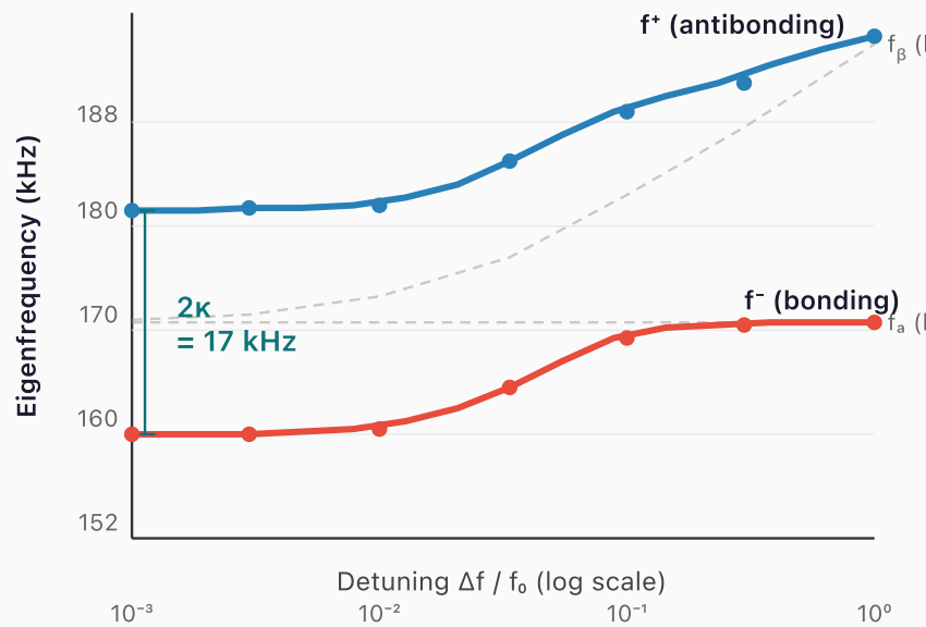
(a) Avoided Crossing: Eigenfrequencies vs. Detuning
