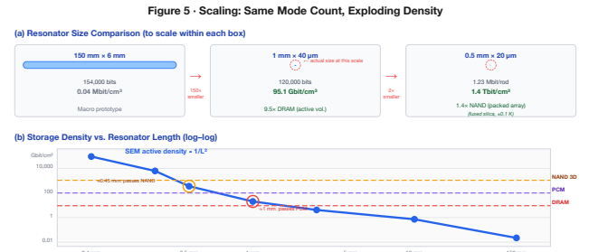
Figure 5. (a) Size comparison at three scales: the 150 mm macro prototype (0.04 Mbit/cm³), the 1 mm borosilicate MEMS rod (95.1 Gbit/cm³ active, 9.5× DRAM), and a 0.5 mm fused silica array (1.4 Tbit/cm³ packed-array, 1.4× NAND Flash). All designs share the same thermally stable mode physics. (b) Log-log density vs. rod length showing CWM crossing DRAM at 2.1 mm, PCM at 1.15 mm, and NAND Flash at 0.45 mm—all within standard MEMS fabrication range.
