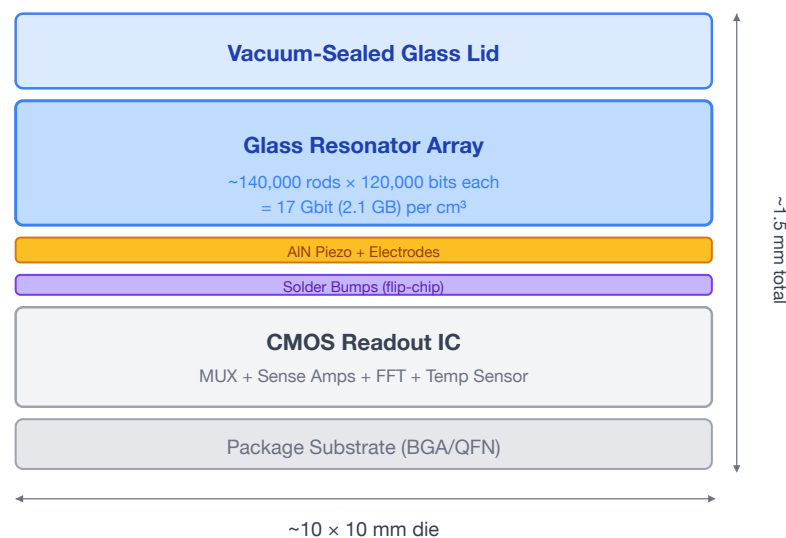
Figure 2. MEMS resonator at chip scale. (a) Cross-section of a single 1 mm × 40 μm glass resonator element showing AIN piezo transducers, anchor tethers, vacuum cavity, and lithographic mass perturbations. (b) Scale comparison: the rod diameter (40 μm) is thinner than a human hair (70 μm). (c) Top-down view of a resonator array at 80 μm pitch on a CMOS readout die. (d) Chip integration stack: vacuum-sealed glass array flip-chip bonded to CMOS — identical to existing MEMS accelerometer packaging.
