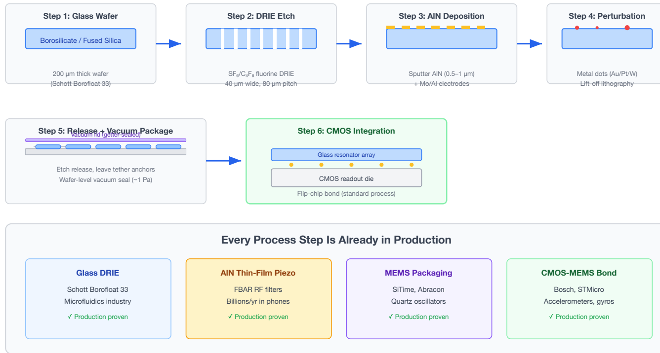
Figure 6. CWM fabrication process flow. Six steps — all using processes already in volume production. Glass DRIE is used in microfluidics (Schott Borofloat 33); AlN thin-film piezo is in billions of smartphone FBAR filters; MEMS vacuum packaging is standard for oscillators and gyroscopes (SiTime, Abracon); CMOS-MEMS flip-chip bonding is used in Bosch and STMicro accelerometers. The innovation is the architectural combination, not the fabrication.
