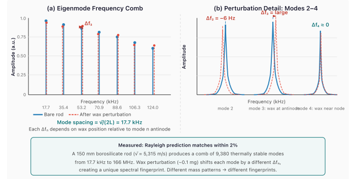
Figure 5. (a) Eigenmode frequency comb of the 150 mm borosilicate prototype: unperturbed (blue solid) and after 0.1 mg wax perturbation (red dashed). Each mode shifts by a different \Delta f_n depending on the wax position relative to that mode’s antinode. (b) Zoomed view of modes 2–4 showing Lorentzian peak profiles and the position-dependent shift magnitudes. Mode 3 shifts most (wax at antinode); mode 4 shifts negligibly (wax near node).
