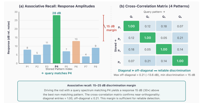
Figure 7. (a) Response amplitudes when querying for pattern P4 across an 8-rod array. The matching rod produces a 28 dB response—15 dB above the best non-matching pattern (P6), providing a 30× power margin for reliable detection. (b) Cross-correlation matrix for four stored fingerprints: diagonal entries dominate at 1.00, off-diagonal entries ≤ 0.21, confirming spectral orthogonality.
