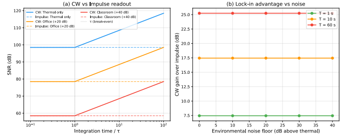
Figure 3. (a) CW lock-in readout exceeds impulse SNR for integration times beyond \tau , with gain independent of noise environment. (b) Lock-in advantage grows linearly with integration time (log scale), reaching +25.2 dB at 60 s for the 150 mm borosilicate reference rod ( \tau = 180 ms, Q = 10,000 ).
