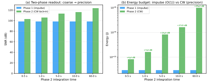
Figure 4. Two-phase readout architecture: Phase 1 (broadband impulse) performs parallel search across all rods in one ring-down time \tau ; Phase 2 (CW lock-in) provides precision measurement on the winning rod at +17.5 dB SNR gain.
