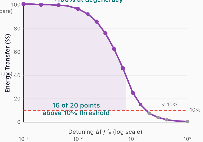
(b) Hybridisation Depth vs. Detuning ~100% at degeneracy
