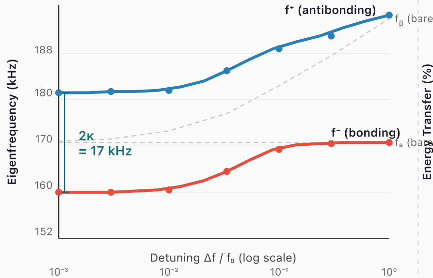
(a) Avoided Crossing: Eigenfrequencies vs. Detuning
