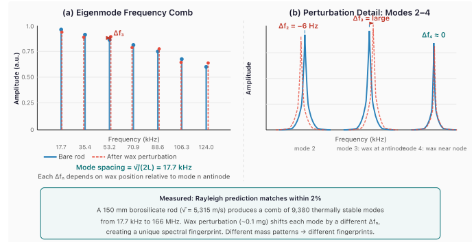
Figure 11. (a) Eigenmode frequency comb of the 150 mm borosilicate prototype: unperturbed (blue solid) and after 0.1 mg wax perturbation (red dashed). Each mode shifts by a different \Delta f_n , depending on the wax position relative to that mode's antinode. (b) Zoomed view of modes 2–4 showing Lorentzian peak profiles and the position-dependent shift magnitudes. Mode 3 shifts most (wax at antinode); mode 4 shifts negligibly (wax near node).
