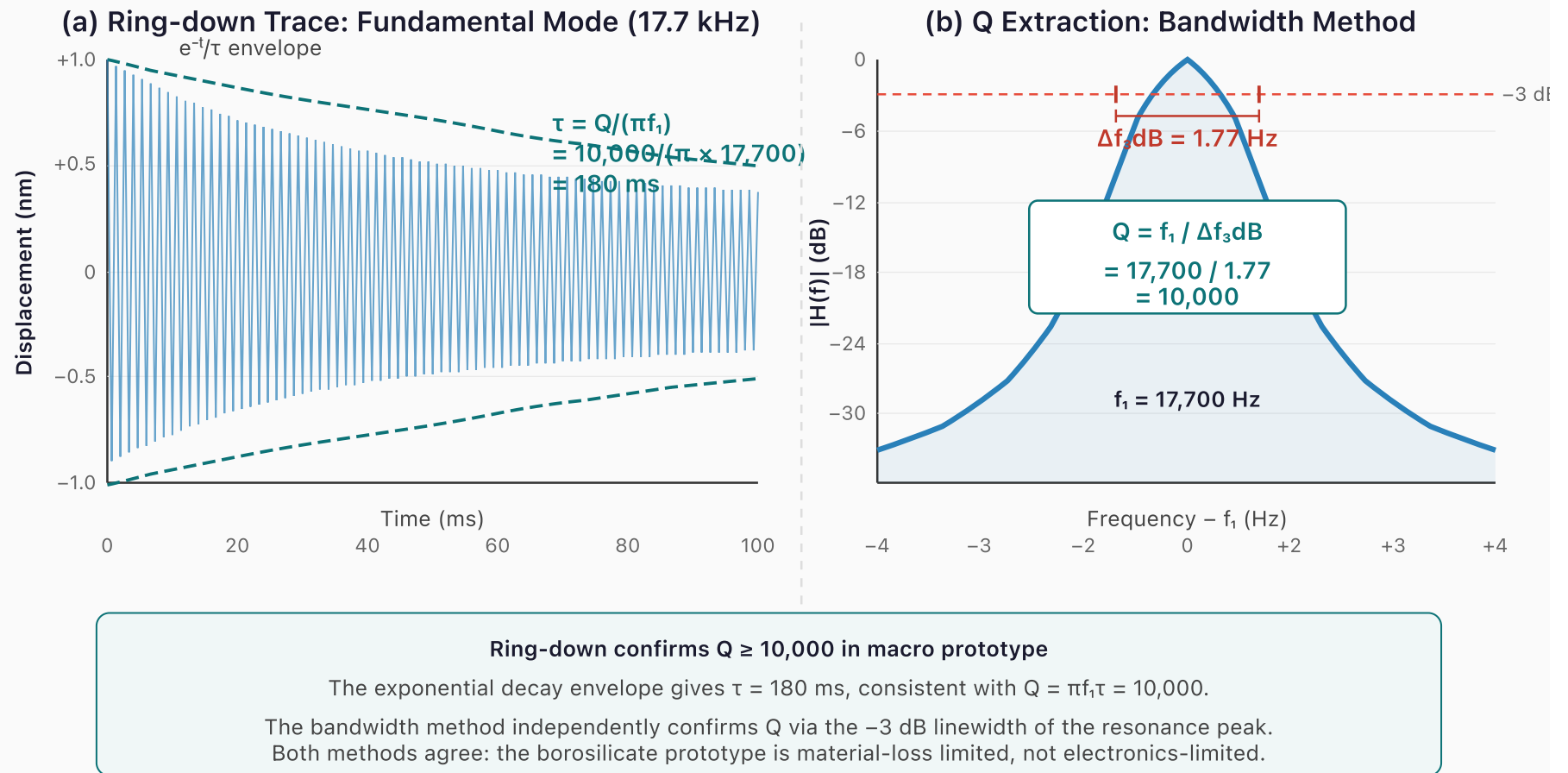
Figure 12. Q-factor measurement of the macro prototype. (a) Ring-down waveform of the fundamental mode (17.7 kHz) after impulse excitation: the exponential envelope decays with \tau = 180 \text{ ms} , giving Q = \pi f_1 \tau = 10,000 . (b) Bandwidth method: the -3 \text{ dB} linewidth of the Lorentzian resonance peak is \Delta f_{3\text{dB}} = 1.77 \text{ Hz} , independently confirming Q = f_1 / \Delta f_{3\text{dB}} = 10,000 . Both methods agree that the prototype is material-loss-limited, not electronics-limited — the USB oscilloscope is not the bottleneck.
