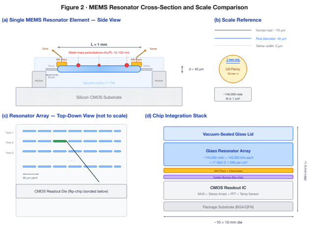
Figure 2. MEMS resonator cross-section showing AlN piezo transducers, anchor tethers, vacuum cavity, and lithographic perturbation masses.
