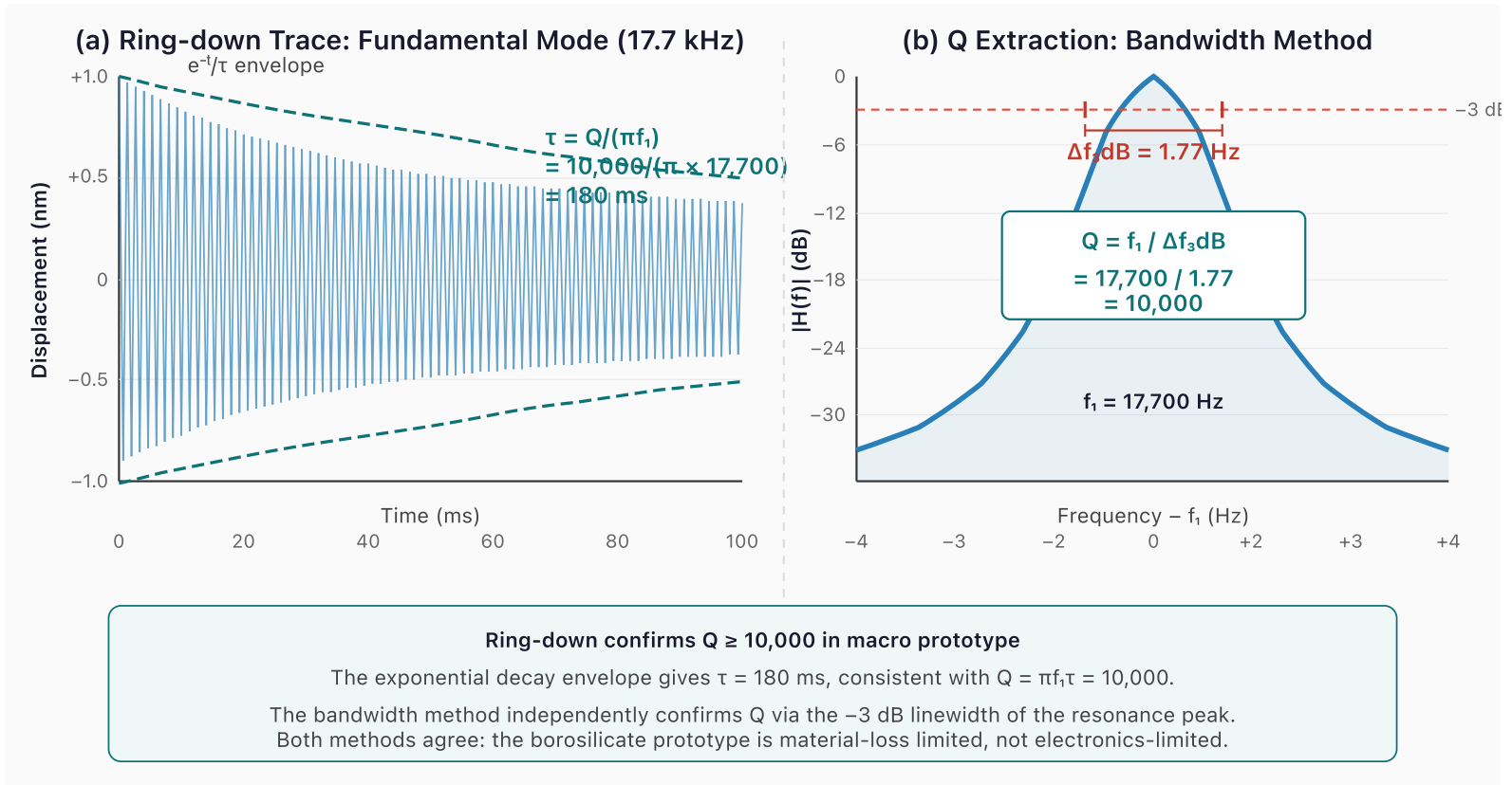
Figure 12. Q-factor measurement of the macro prototype. (a) Ring-down waveform of the fundamental mode (17.7 kHz) after impulse excitation: the exponential envelope decays with \tau = 180 \text{ ms} , giving Q = \pi f_1 \tau = 10,000 . (b) Bandwidth method: the -3 \text{ dB} linewidth of the Lorentzian resonance peak is \Delta f_{3\text{dB}} = 1.77 \text{ Hz} , independently confirming Q = f_1 / \Delta f_{3\text{dB}} = 10,000 . Both methods agree that the prototype is material-loss-limited, not electronics-limited — the $25 USB oscilloscope is not the bottleneck.
