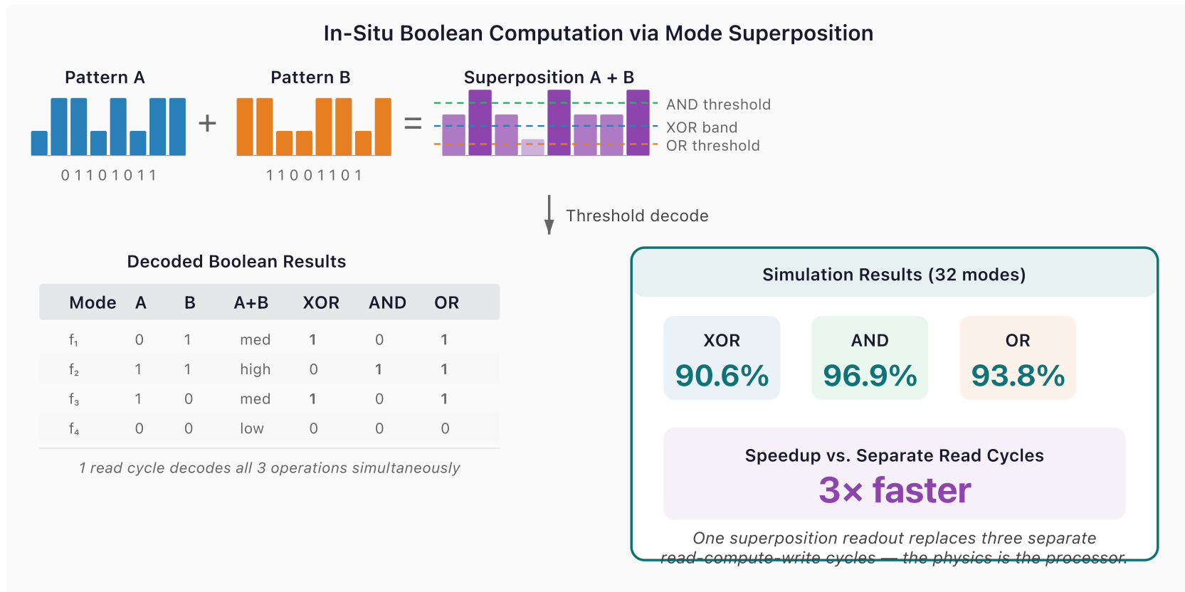
Figure 8. In-situ Boolean computation via mode superposition. Two stored patterns (A, B) are superposed; the combined amplitude distribution is decoded into XOR (90.6% fidelity), AND (96.9%), and OR (93.8%) using amplitude thresholds — all from a single readout cycle. This provides 3× throughput vs. conventional read-compute-write approaches and confirms SEM as a true compute-in-memory technology.
