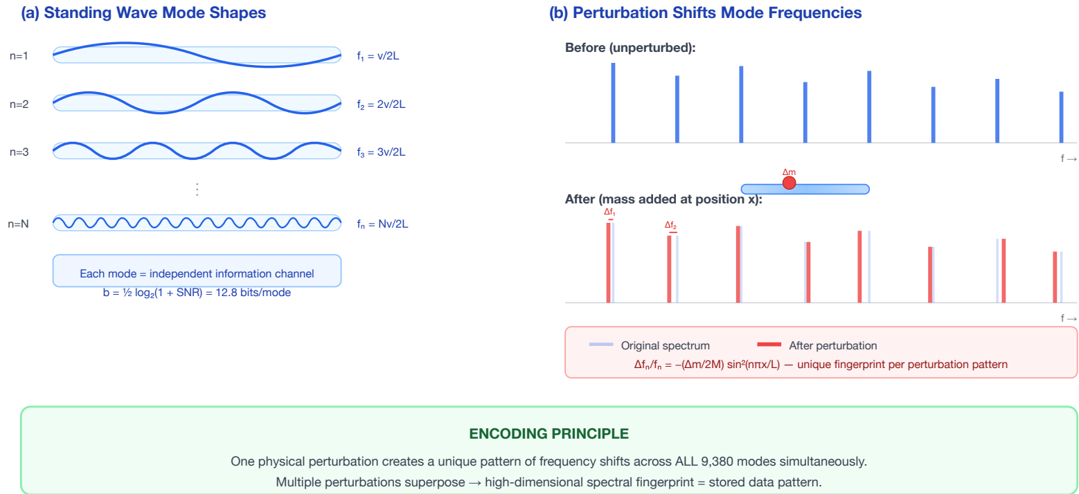
Figure 3. Eigenmode encoding. (a) Standing wave mode shapes for modes n = 1, 2, 3, \dots, N within a glass rod — each mode is an independent information channel at a distinct frequency. (b) Perturbation effect: adding mass at a specific position shifts each mode frequency by a different amount (Rayleigh perturbation formula), creating a unique spectral fingerprint that encodes the perturbation's position and mass.
