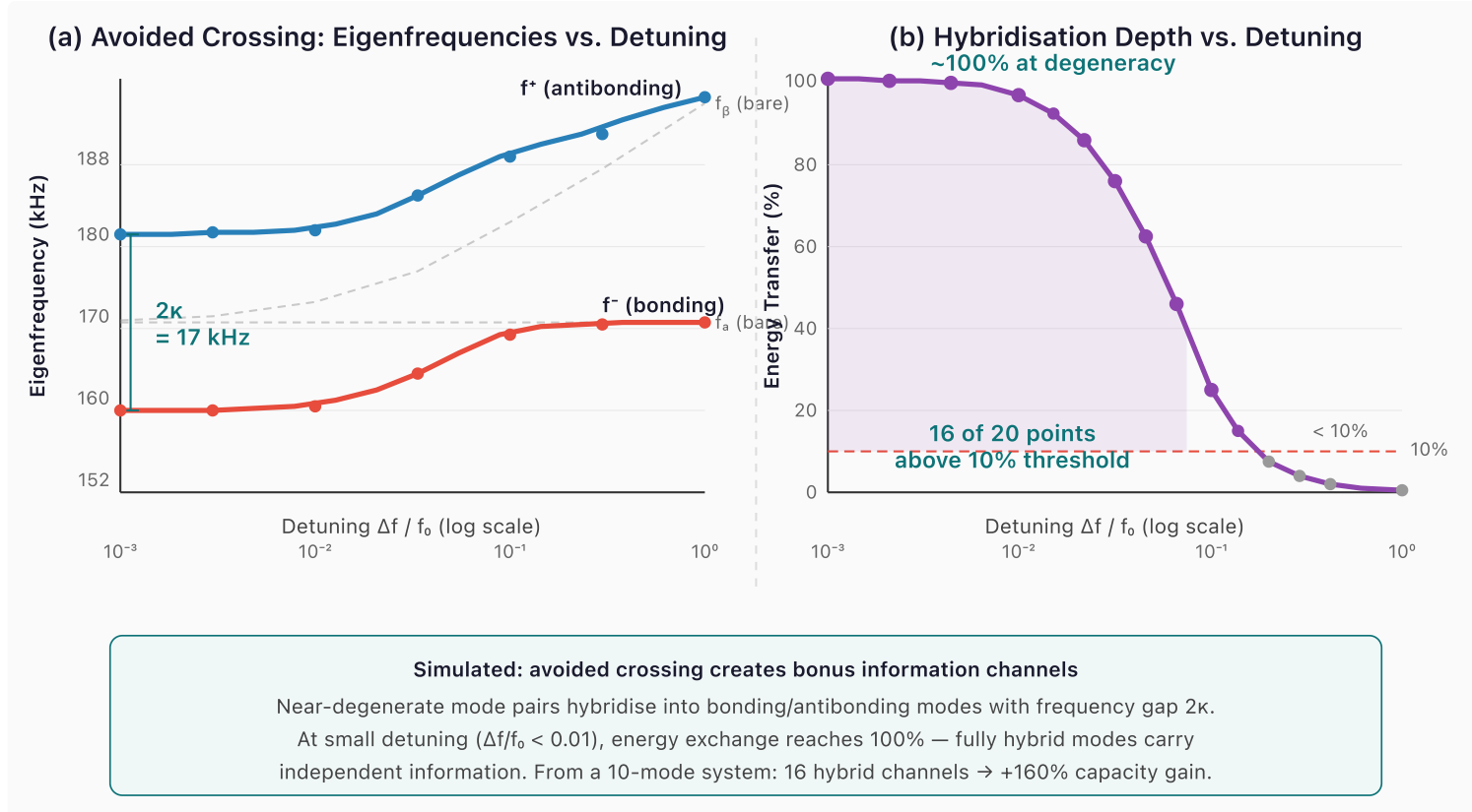
Figure 14. Simulated avoided crossing for two coupled modes ( \kappa = 0.05\omega_0 , f_0 = 170 kHz). (a) Eigenfrequency diagram: uncoupled modes (dashed grey) would cross at zero detuning; coupling creates bonding ( f^- , red) and antibonding ( f^+ , blue) branches separated by minimum gap 2\kappa = 17 kHz. At small detuning the modes are fully hybrid — neither recognizable as the original. (b) Hybridization depth vs. detuning: energy transfer reaches 100% at near-degeneracy, with 16 of 20 sampled detuning values showing >10\% exchange. Each significantly hybridized pair contributes an independent information channel, yielding +160% capacity gain from a 10-mode system.
