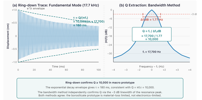
Figure 12. (a) Ring-down waveform of the fundamental mode (17.7 kHz) after impulse excitation. The exponential envelope decays with \tau = 180 \text{ ms} , corresponding to Q = 10,000 . (b) Frequency-domain measurement: the -3 \text{ dB} bandwidth of the Lorentzian resonance peak is 1.77 Hz, independently confirming Q = f_1/\Delta f_{3\text{dB}} = 10,000 . Both methods agree that the prototype is material-loss-limited.
