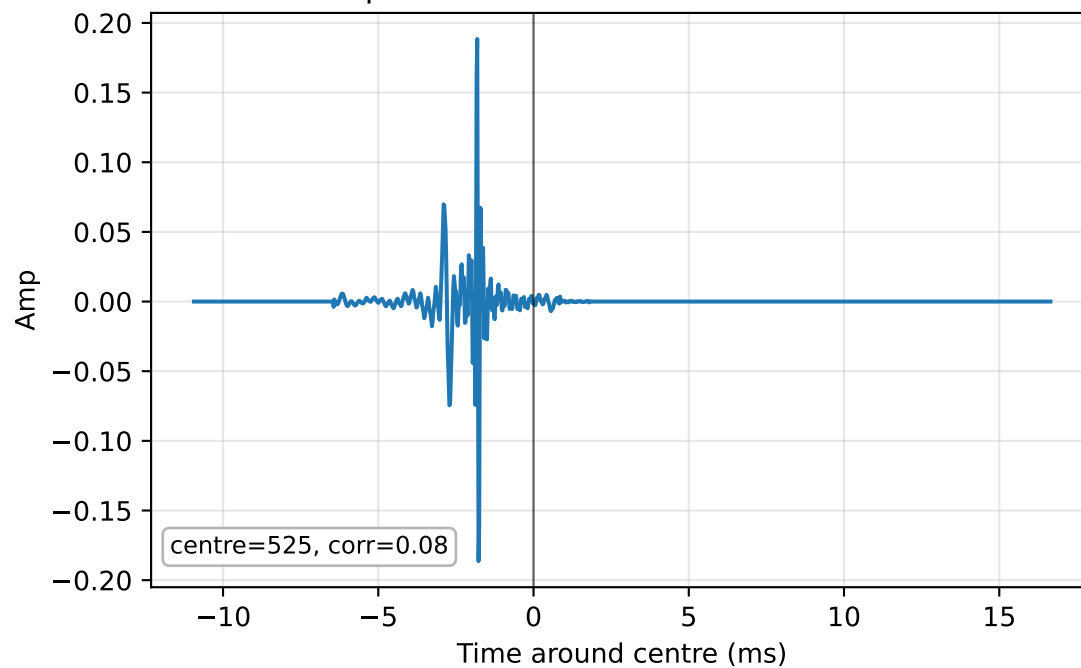
Zw impulse — zoom around detected centre
