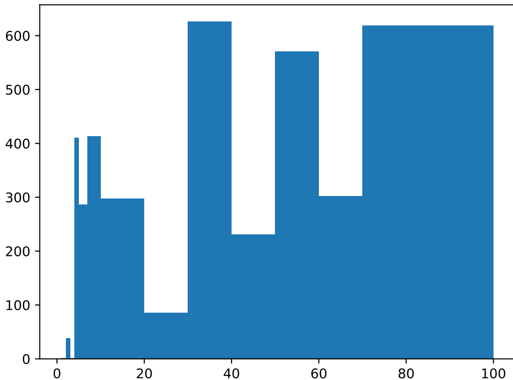
Crystalline domain size distribution, PVA-100, time 13200000, \phi = 0.372
