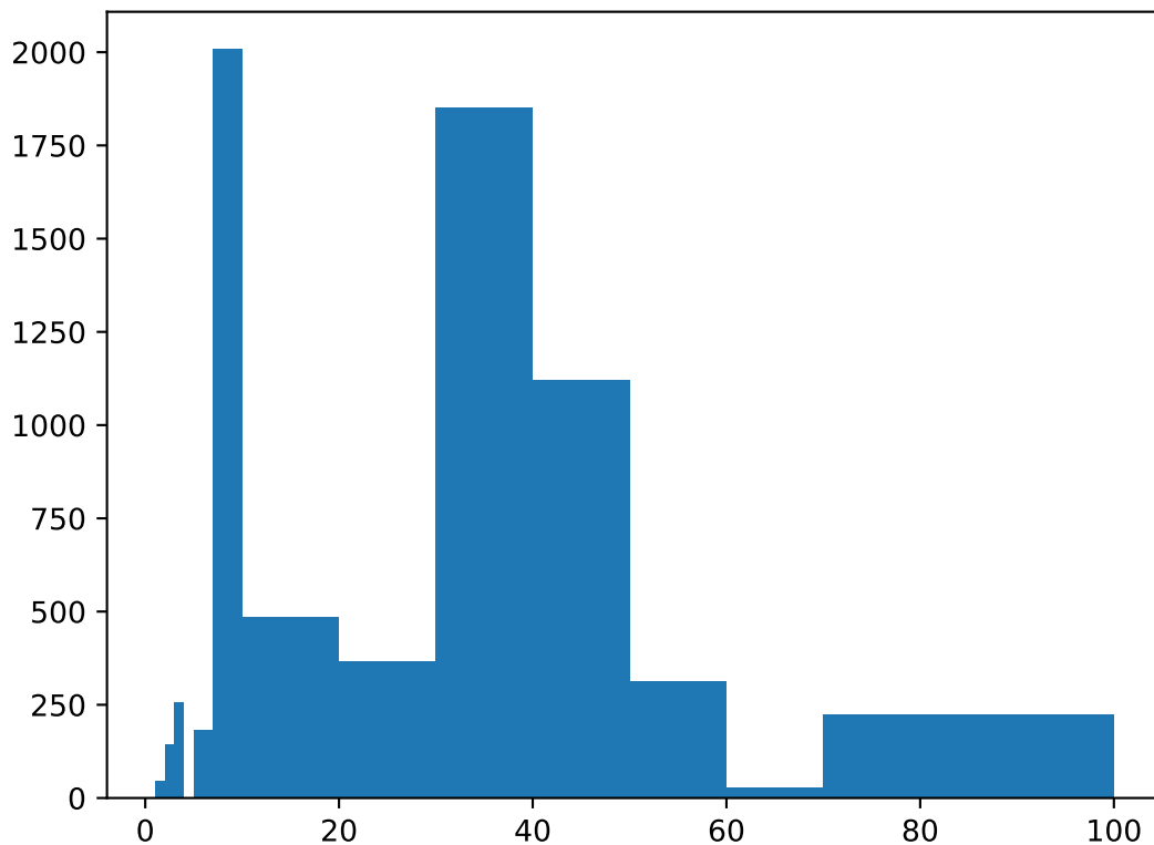
Crystalline domain size distribution, PVA-100, time 36000000, \phi = 0.440
