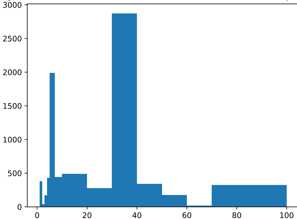
Crystalline domain size distribution, PVA-100, time 600000000, \phi = 0.460
