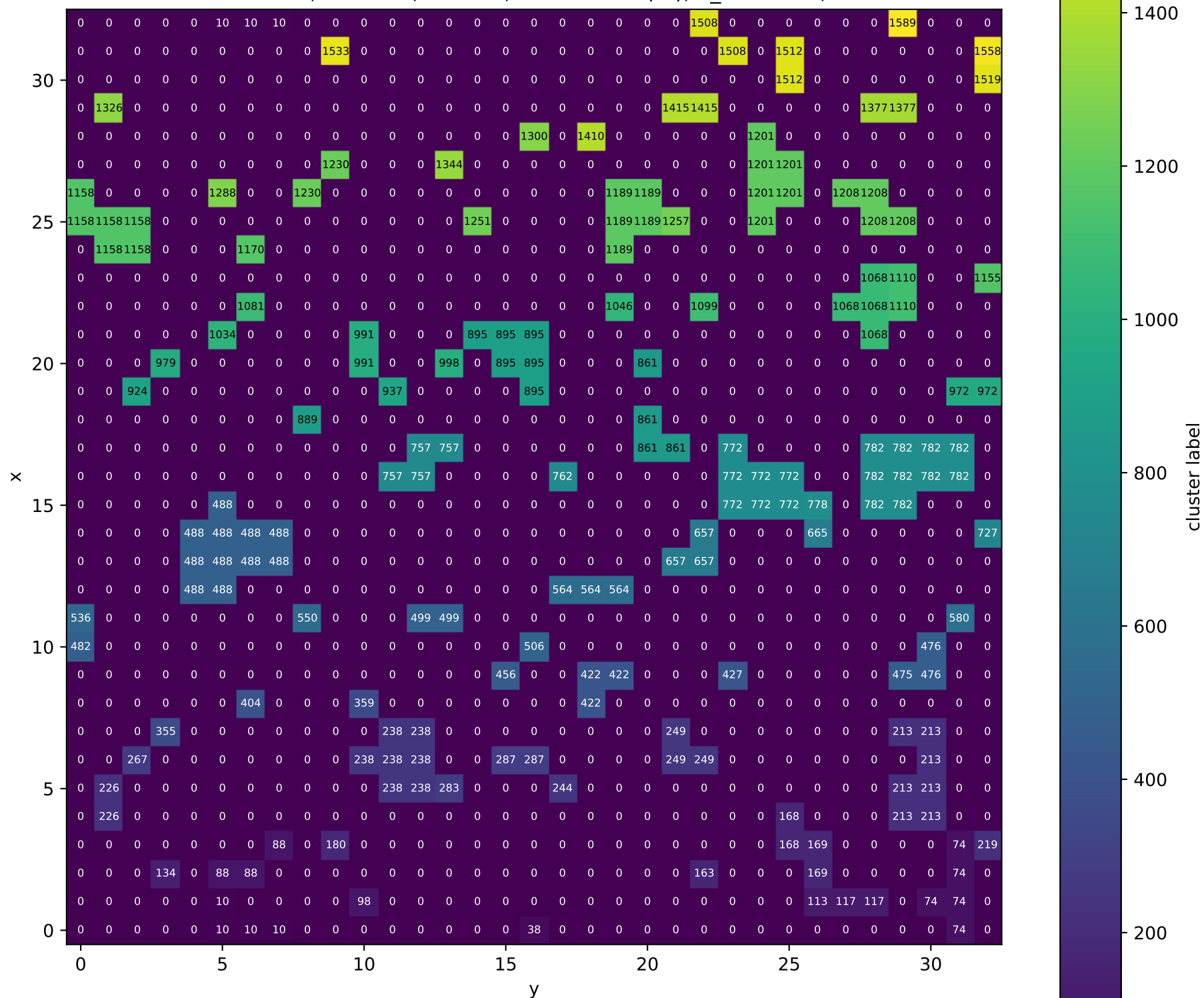
Cluster labels, PVA-100, T = 0.5 , T_{dot} = 10^{**}(-5) , T_{init} = 1.0 , z = 25
