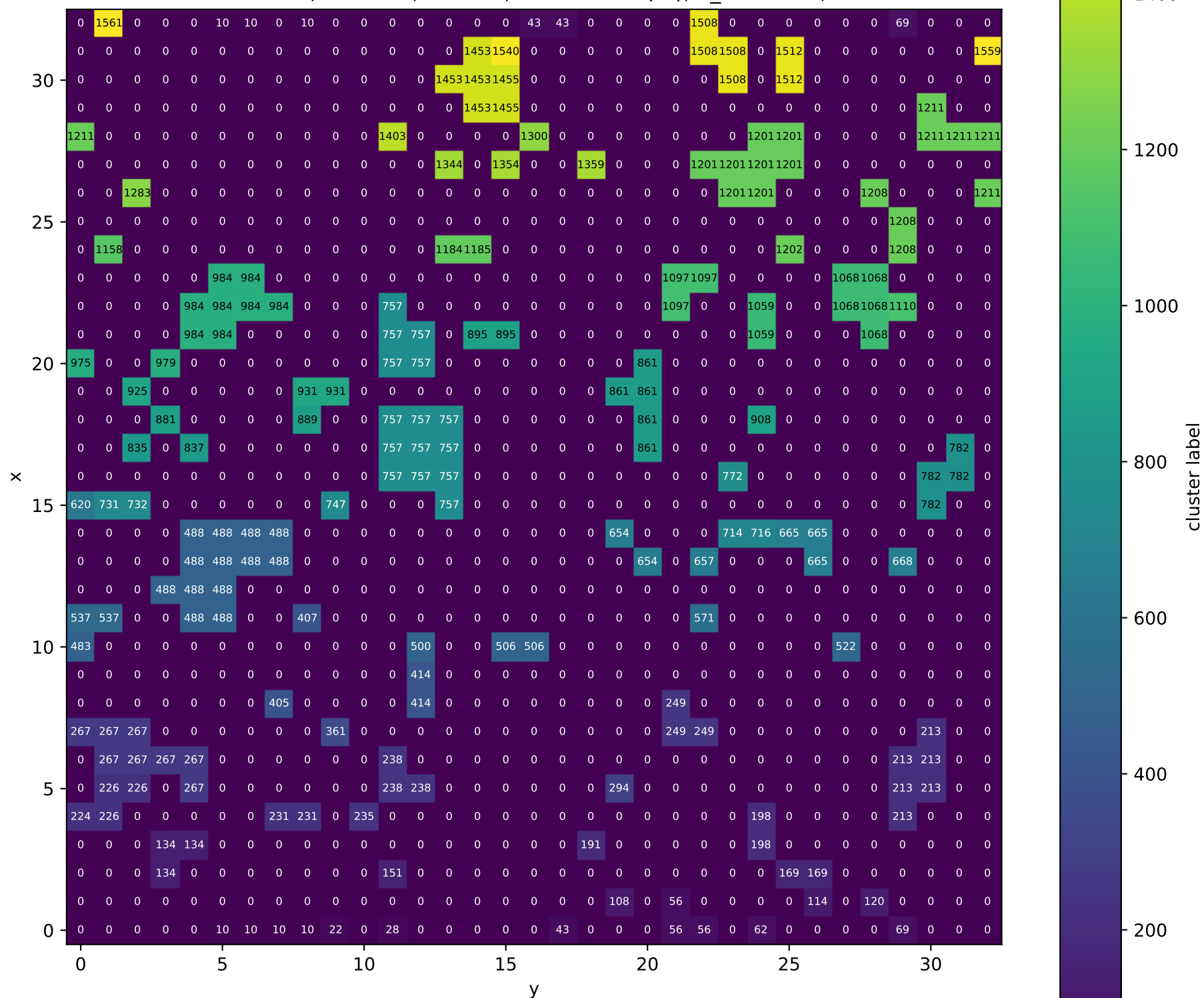
Cluster labels, PVA-100, T = 0.5 , T_{\text{dot}} = 10^{*(-5)} , T_{\text{init}} = 1.0 , z = 26
