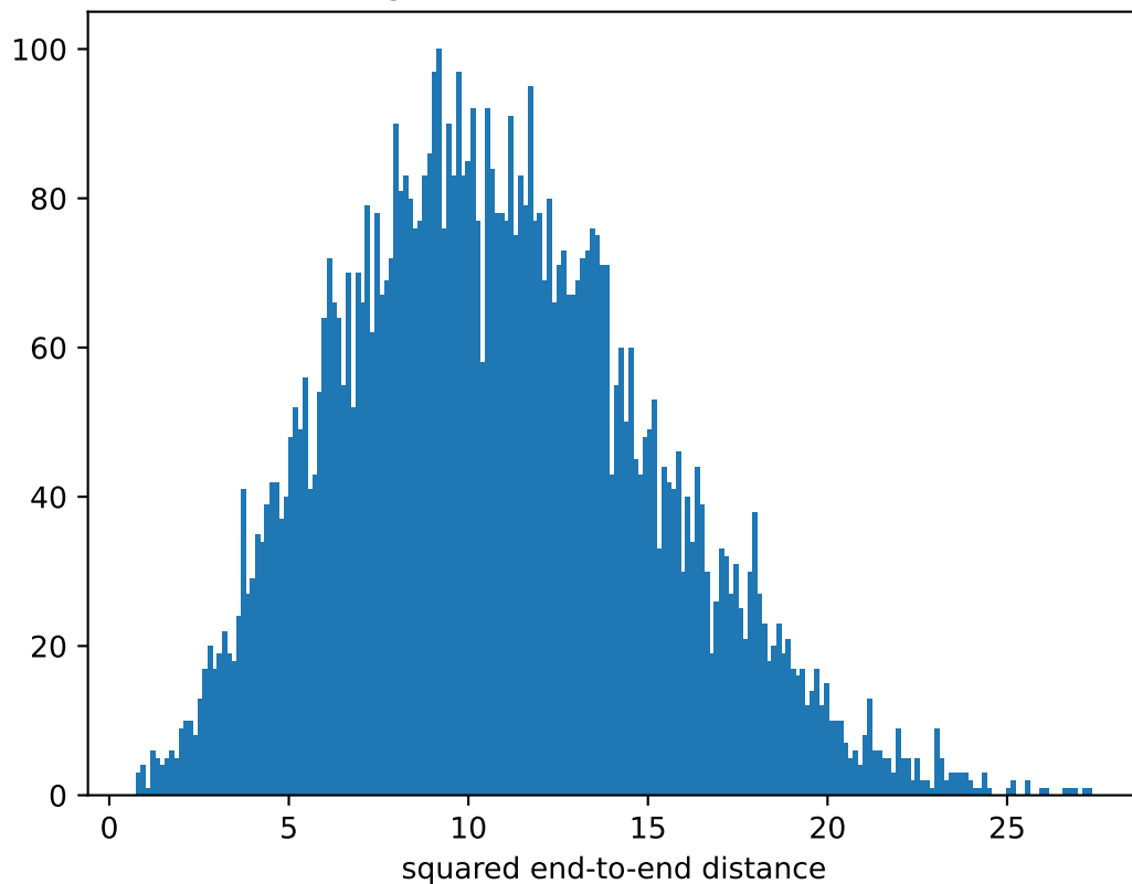
End-to-end length distribution, PVA-100, \dot{T} = 10^{-5} , T = 1
