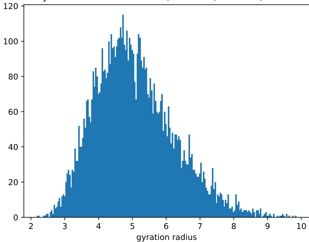
Gyration radius distribution, PVA-100, \dot{T} = 10^{-5} , T = 0.5
