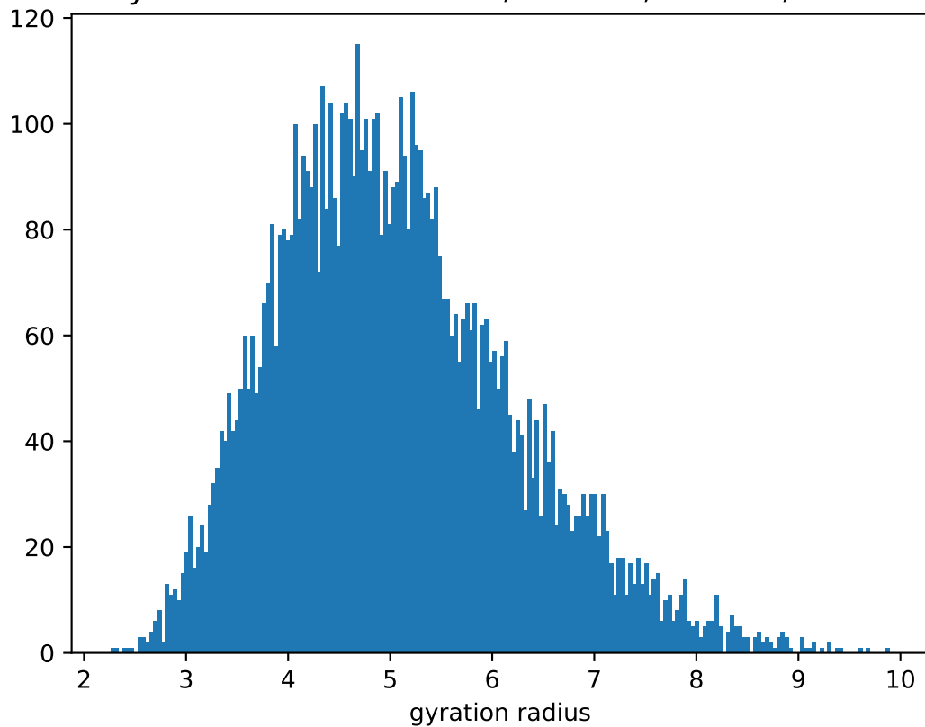
Gyration radius distribution, PVA-100, \dot{T} = 10^{-5} , T = 0.7
