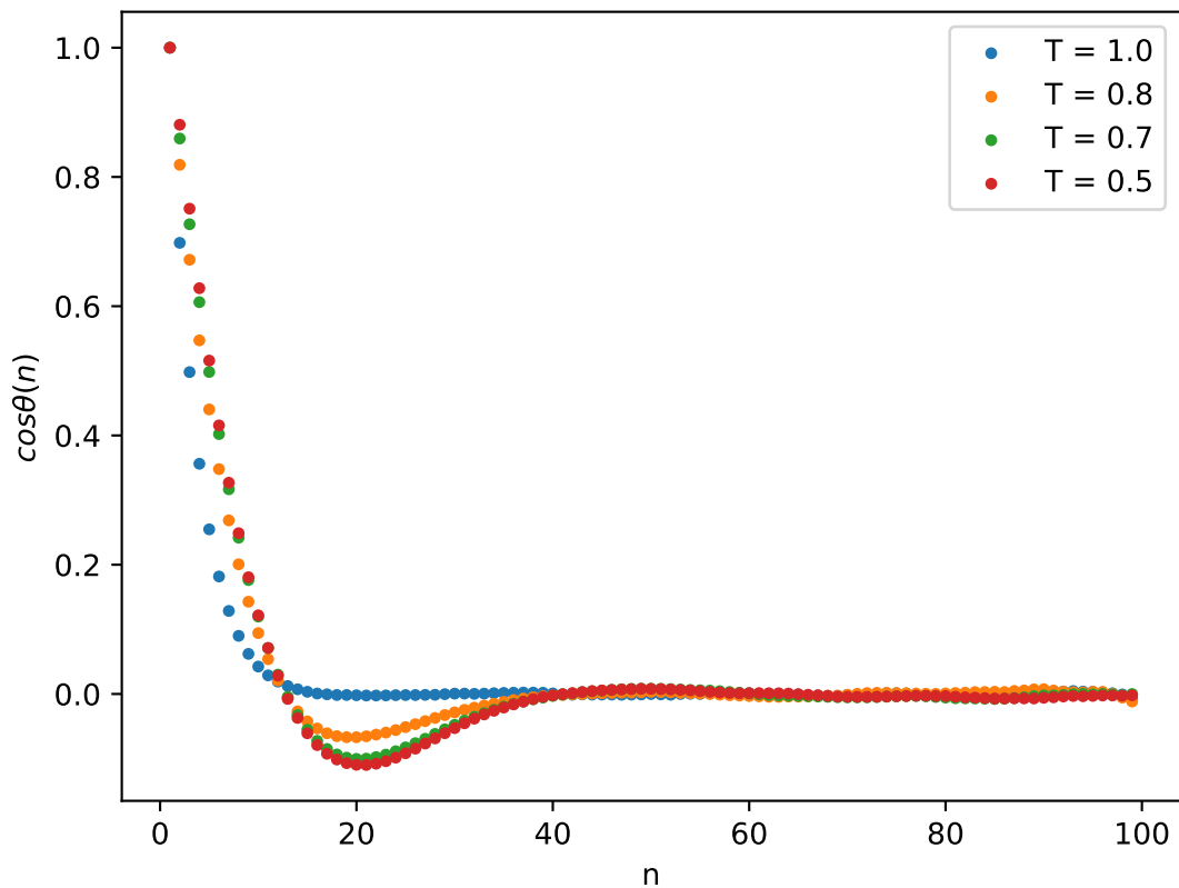
Distribution of bond-bond correlations, PVA-100, \dot{T} = 10^{-5}
