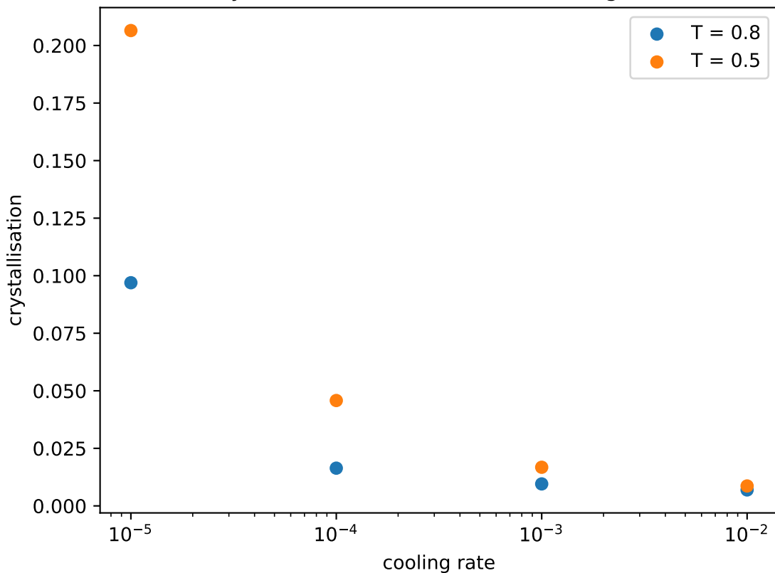
Crystallisation as function of cooling rate
