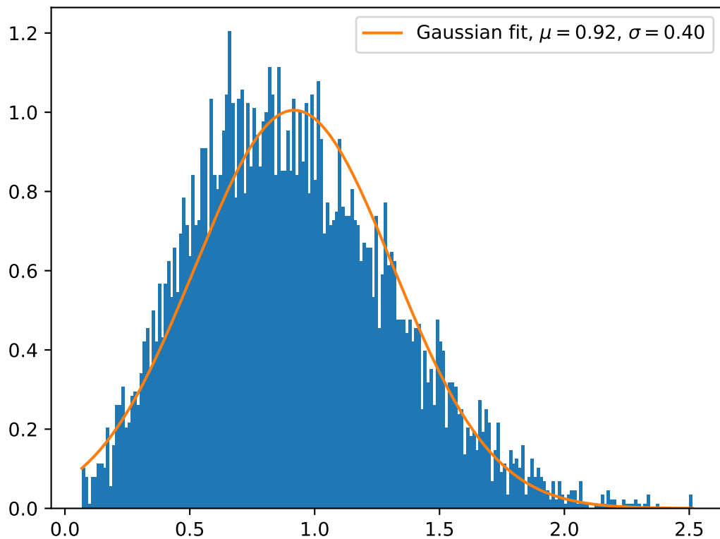
Distribution of end-to-end distance, PVA-100, simulation start
